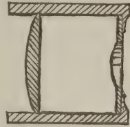
THE HUYGHENIAN EYE-PIECE
